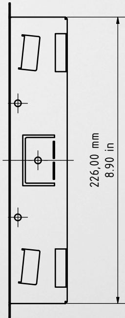
Flush-mounting housing (backbox)
