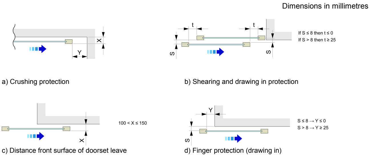
Figure 2 — Examples of safety distances for sliding doorsets
