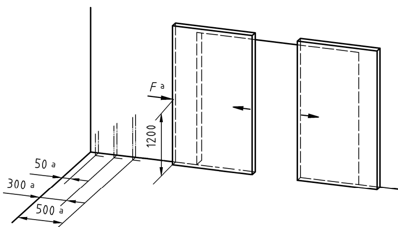
Figure B.1 — Single-leaf sliding doorset
